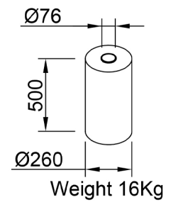
Stretch film spool dimension
